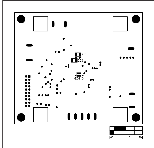
Figure 7. MAX1645B EV Kit Component Placement Guide—Solder Side
