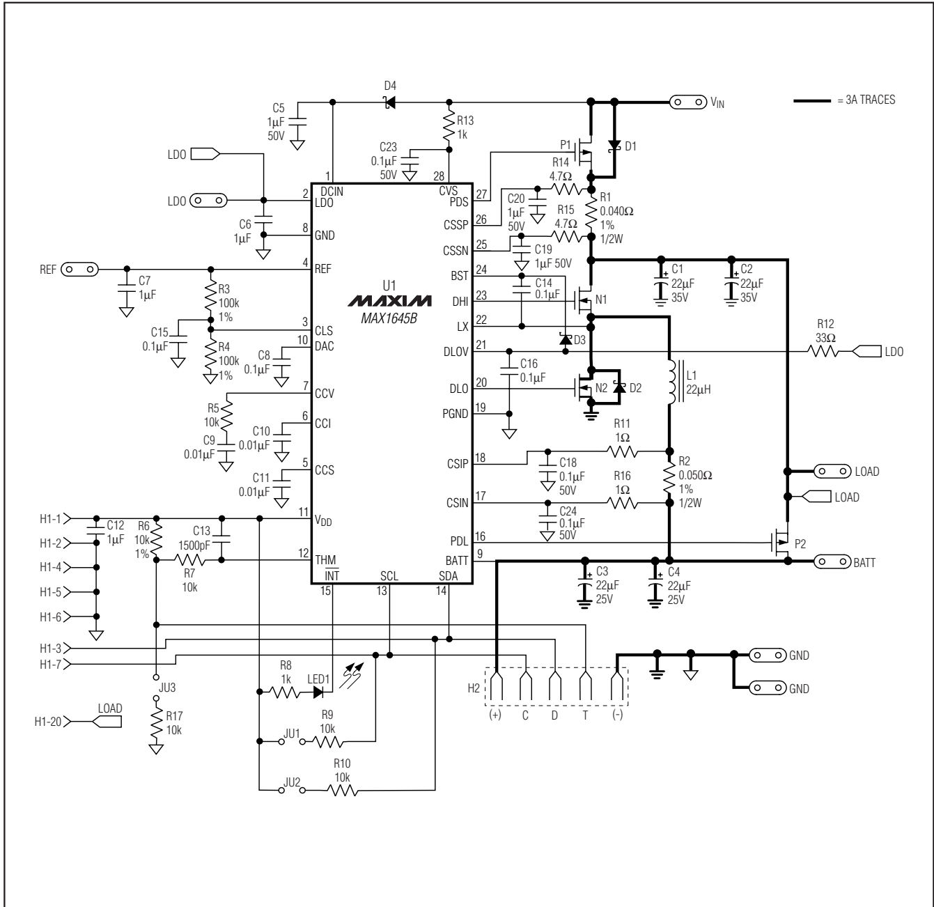
Figure 5. MAX1645B EV Kit Schematic
