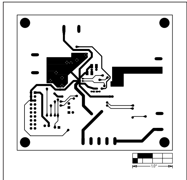
Figure 9. MAX1645B EV Kit PC Board Layout—Solder Side
